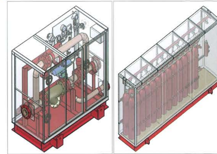
Deluge Valve Skid 3-D Modelling
